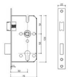
Croos Section Diagrams & Measurements for 58 Dead Lock LBK锁体，尺寸图/开孔图
