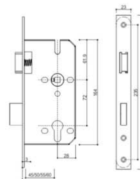
Croos Section Diagrams & Measurements for 72 Dead Lock LBK锁体，尺寸图/开孔图
