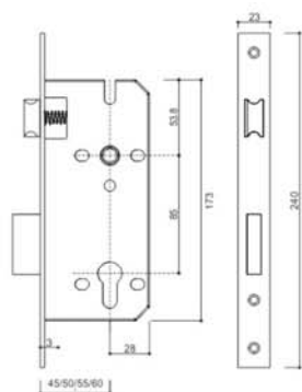
Croos Section Diagrams & Measurements for 85 Dead Lock LBK锁体，尺寸图/开孔图
