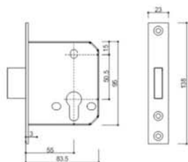
Croos Section Diagrams & Measurements for 55 Dead Lock LBK锁体, 尺寸图/开孔图
