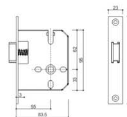
Croos Section Diagrams & Measurements for 55 Dead Lock LBK锁体, 尺寸图/开孔图
