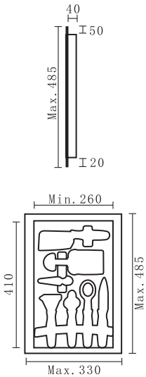
套装器具盘 Cutlery tray
