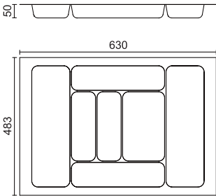
刀叉盘 Cutlery tray
