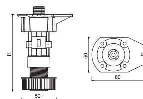
欧式平头可调脚 European adjustable feet
