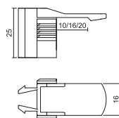
可调脚卡扣 (配木踢脚板) Adjustable feet clip
