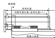
高深骑马抽 High drawer
