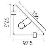
多功能可调脚 Multifunctional adjustable feet
